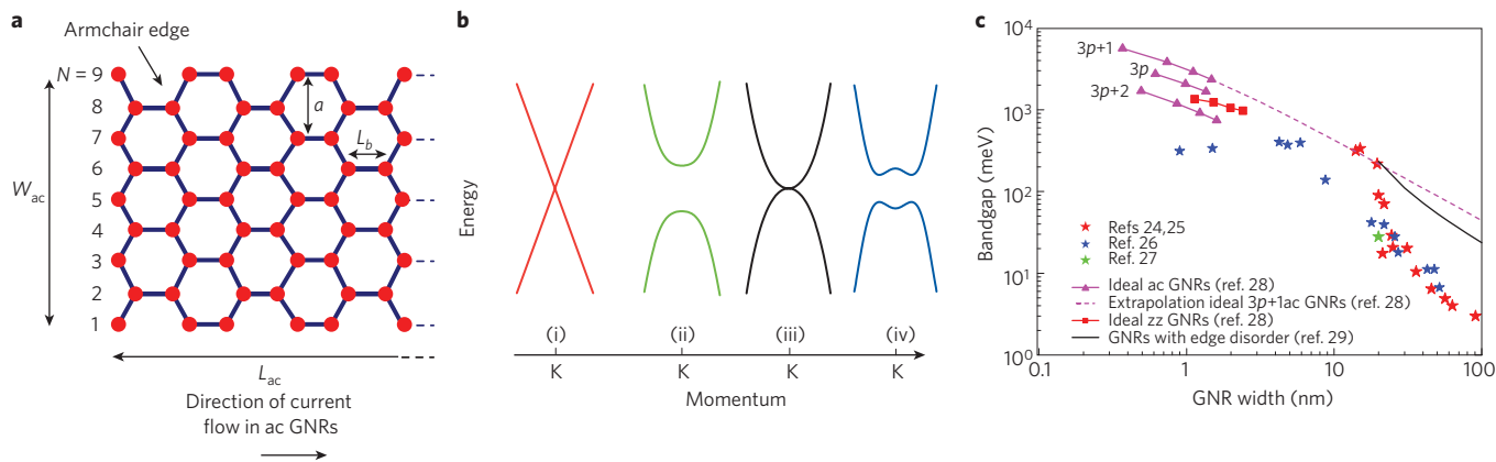
Figure 4 | Properties of graphene and graphene nanoribbons. a , Schematic of an armchair (ac) graphene nanoribbon (GNR) of length L_{ac} and width W_{ac} . The nanoribbon shown here has N = 9 carbon atoms along its width and thus belongs to the 3p family, where p is an integer. b , Band structure around the K point of (i) large-area graphene, (ii) graphene nanoribbons, (iii) unbiased bilayer graphene, and (iv) bilayer graphene with an applied perpendicular field. Large-area graphene and unbiased bilayer graphene do not have a bandgap, which makes them less useful for digital electronics. c , Bandgap versus nanoribbon width from experiments 24–27 and calculations 28,29 . By comparison, the bandgap of Si is above 1 eV. zz: zigzag.
