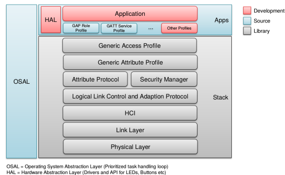
FIGURE 13 – Structure d'un programme
