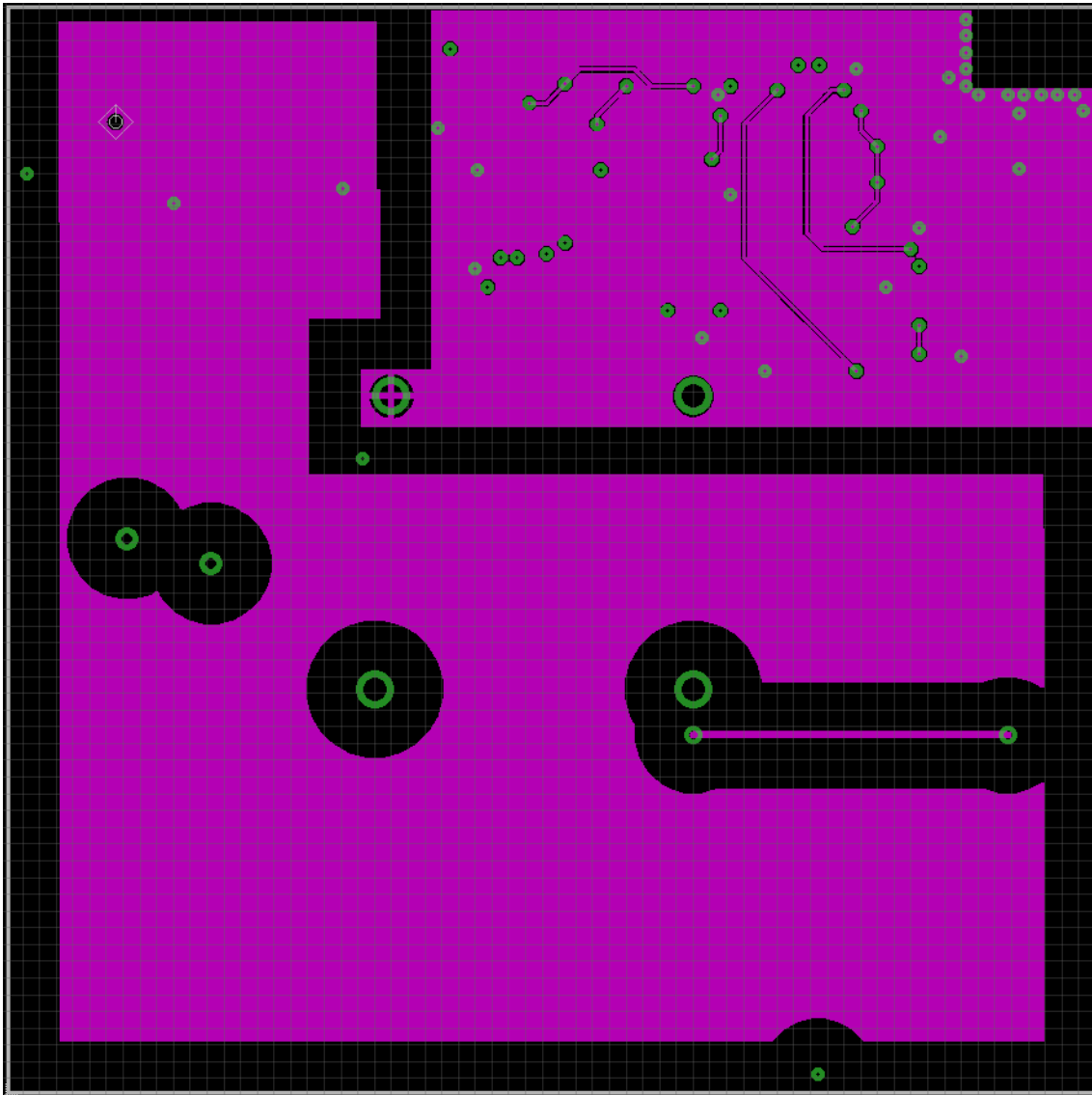
FIGURE 18 – Inner Layer 2
