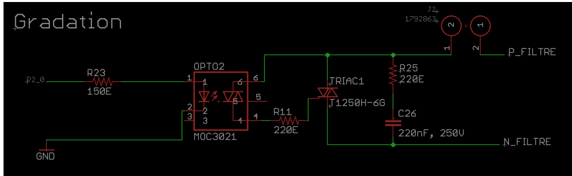
FIGURE 8 – Gradateur
