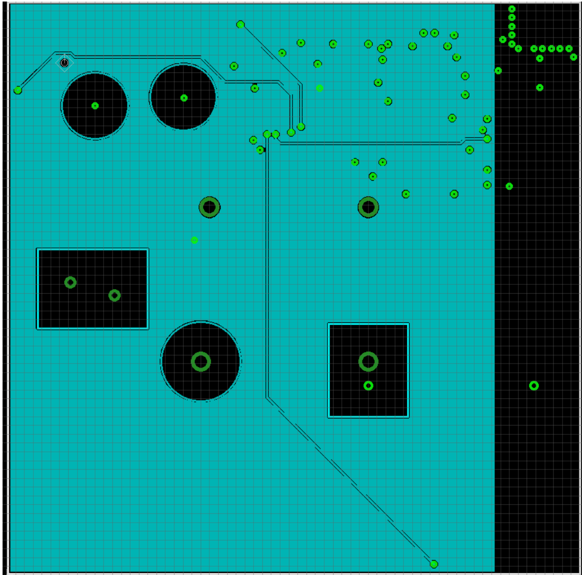
FIGURE 17 – Inner Layer 1
