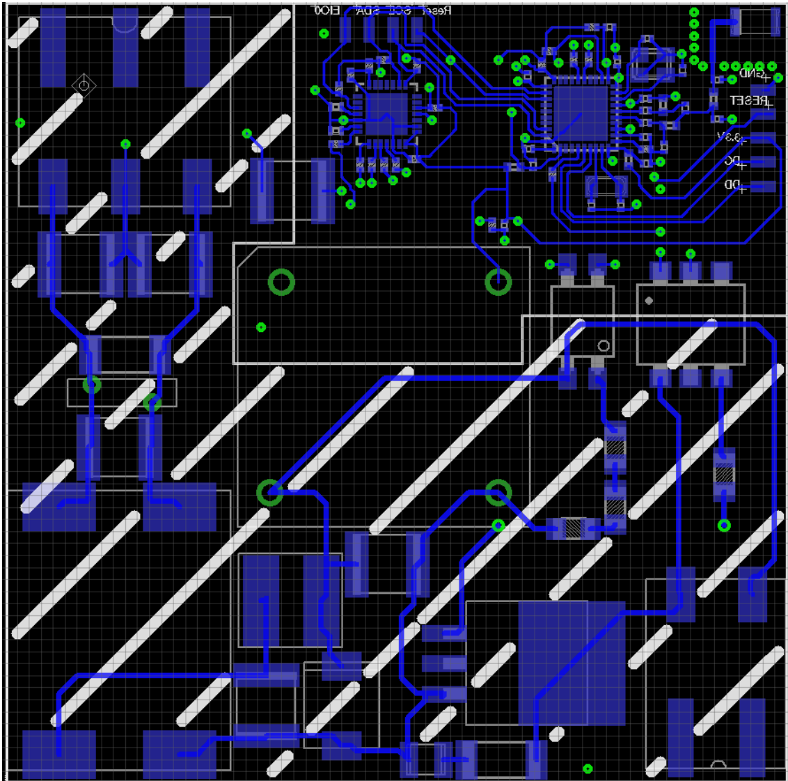
FIGURE 19 – Bottom + sérigraphie + placement composants
