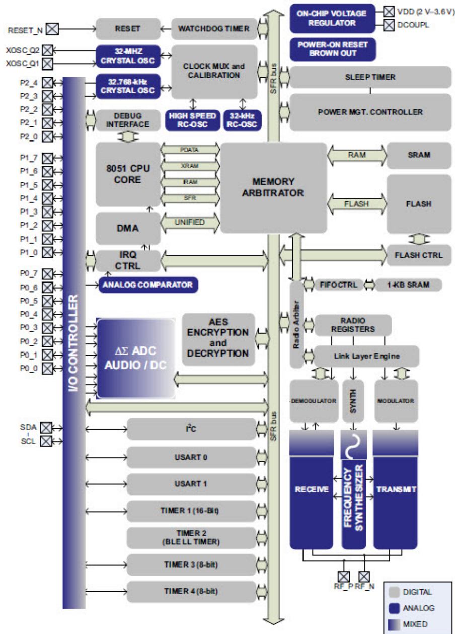
FIGURE 12 – Schéma bloc CC2541
