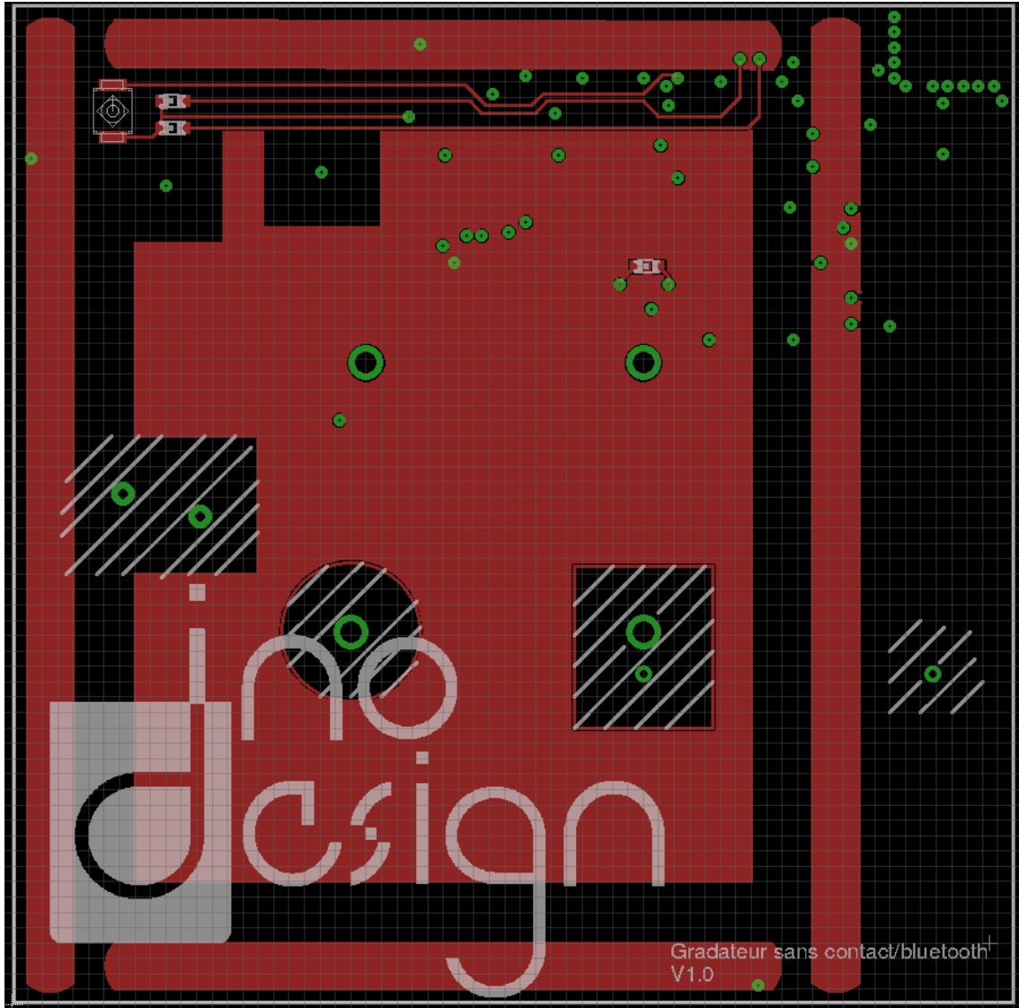
FIGURE 16 – Top + sérigraphie + placement composants
