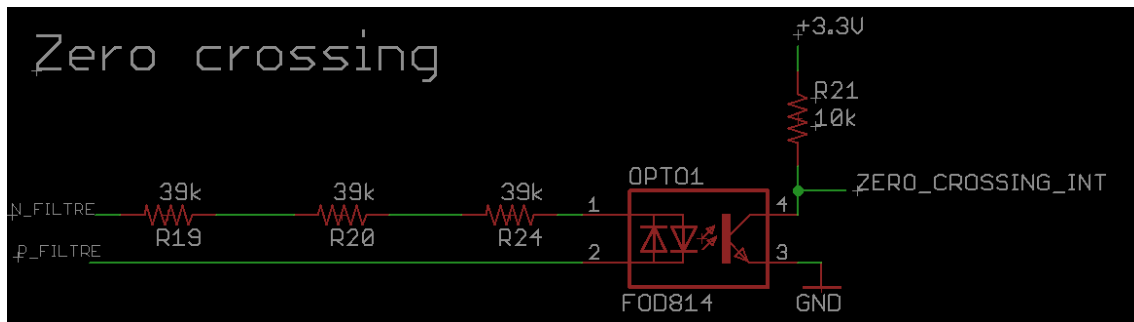
FIGURE 6 – Zero crossing
